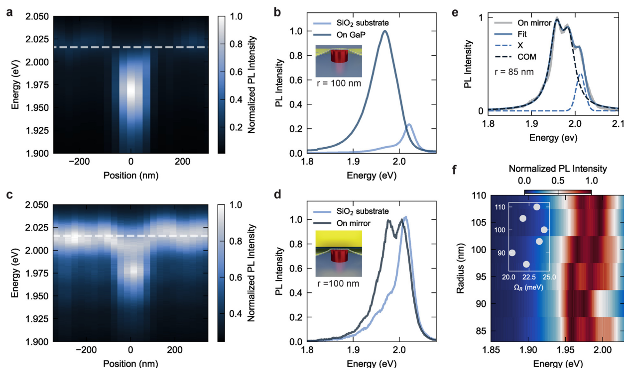
Fig. 3 (a) Room-temperature hyperspectral PL emission map for a WS 2 monolayer coupled to a GaP nanoantenna with 100 nm radius. The excitation laser is scanned linearly across the nanoantenna position, centered at x = 0 nm. (b) Comparison of PL spectra for the uncoupled exciton on a SiO 2 substrate to that from the exciton coupled to the GaP nanoantenna, with the latter exhibiting the expected strain-induced red shift and broadening. The spectra are normalized to the coupled emission intensity maximum. (c) WS 2 hyperspectral PL emission map from the same nanoantenna shown in (a) but with the presence of the gold mirror to generate the nanocavity gap. (d) PL spectrum for the uncoupled exciton on the SiO 2 substrate (at x = 250 nm) compared to the emission at the nanogap position (at x = 0 ), revealing characteristic splitting for the coupled exciton emission. The spectra are normalized to the coupled emission intensity maximum. (e) PL spectrum from monolayer WS 2 embedded in a hybrid nanocavity with GaP nanoantenna radius of 85 nm. The spectrum is fitted with a coupled oscillator model (COM) following eqn (4) (black dashed line), along with a Gaussian peak (blue dashed line) that accounts for the uncoupled and unstrained exciton emission peak (X) (see also ESI note 6†). (f) PL emission from monolayer WS 2 in hybrid nanocavities comprising GaP nanoantennas with radii from 85 to 110 nm. Inset: Rabi energy ( \Omega_R ) values extracted with the COM model in eqn (4).
