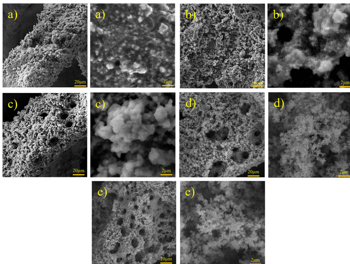
Fig. 2 FESEM images of Ni-Fe-S with magnifications of 10 \times and 100 \times at 10 s, 0.1 M FeSO_4 , and (a) 1, (b) 2, (c) 3, (d) 5, and (e) 6 A cm^{-2} .
