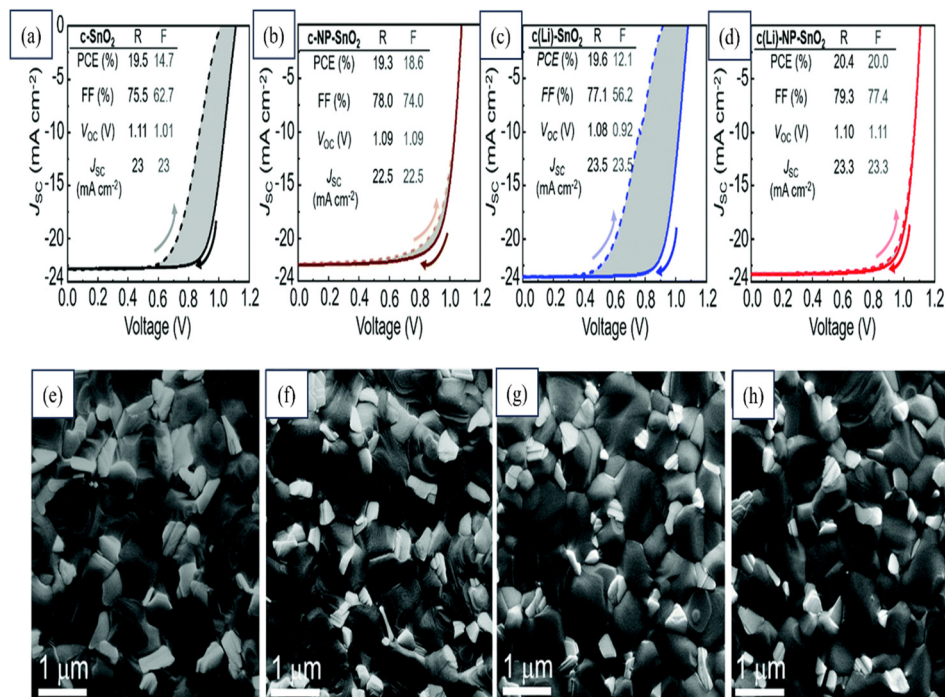
Fig. 21 Reverse (R) and forward (F) J - V scans and stabilized PCE (s-PCE) derived from MPP tracking of champion PSCs with (a) c\text{-SnO}_2 , (b) c\text{-NP-SnO}_2 , (c) c(\text{Li})\text{-SnO}_2 , and (d) c(\text{Li})\text{-NP-SnO}_2 ETLs. Top SEM images of perovskite thin films deposited on (e) c\text{-SnO}_2 , (f) c\text{-NP-SnO}_2 , (g) c(\text{Li})\text{-SnO}_2 , and (h) c(\text{Li})\text{-NP-SnO}_2 ETLs. Reproduced with permission. 200 Copyright 2022, Royal Society of Chemistry.
