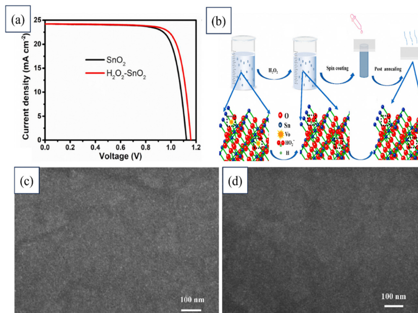
Fig. 22 (a) J - V characteristics of devices with \text{SnO}_2 and \text{H}_2\text{O}_2\text{-SnO}_2 ETLs. (b) Schematic illustration of process used. Top-view SEM images of (c) pristine \text{SnO}_2 film, and (d) \text{H}_2\text{O}_2\text{-SnO}_2 film. Reproduced with permission. 201 Copyright 2021, Elsevier.
