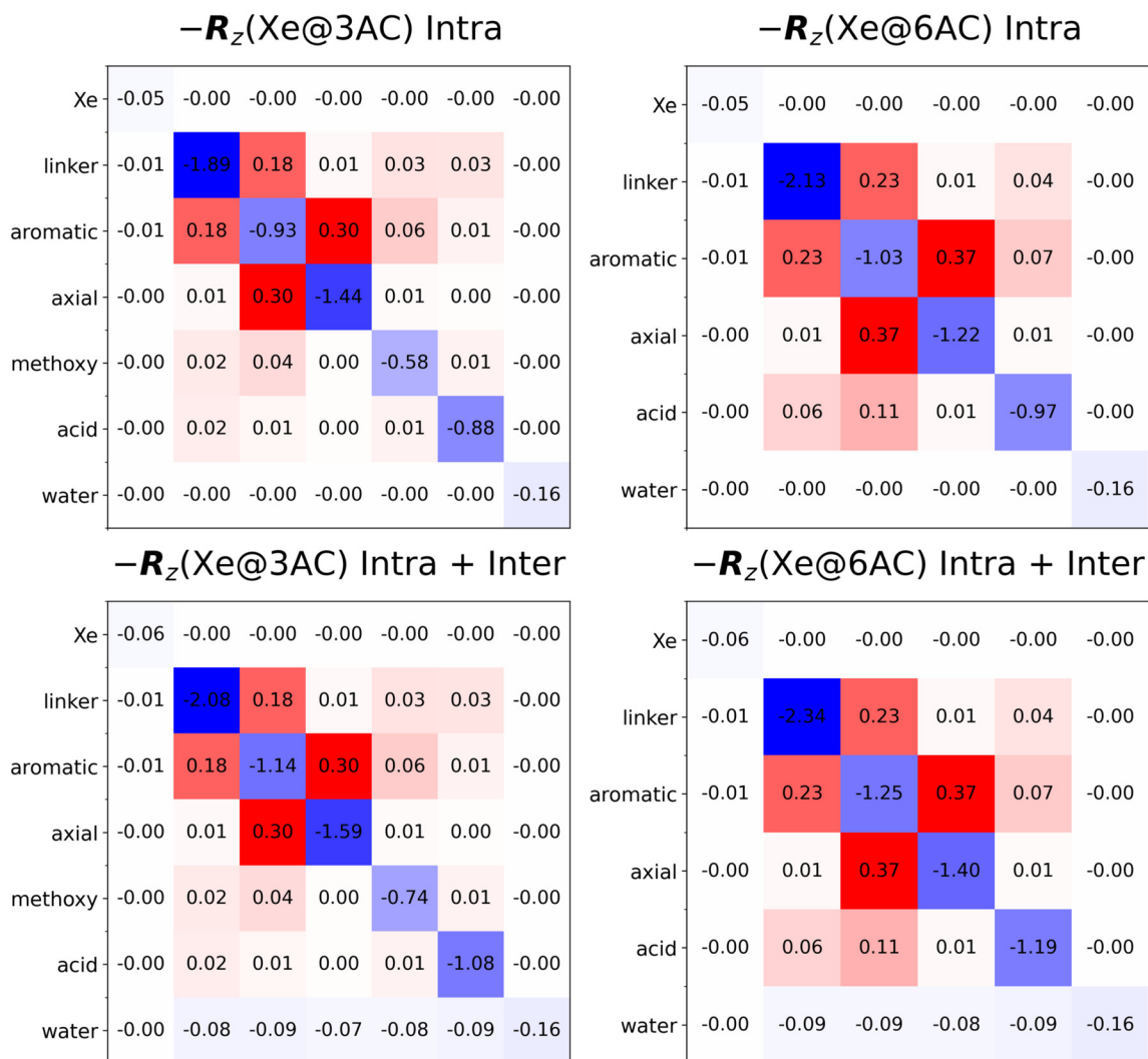
Fig. 2 Longitudinal relaxation matrices, -R_z , for the Xe@Cr(aq) systems (in \text{s}^{-1} ). Intra- and intermolecular (the water solvent) contributions are compared. The values "0.00" correspond to matrix elements with magnitude less than 0.005. The used spin grouping is defined in Fig. 3.
