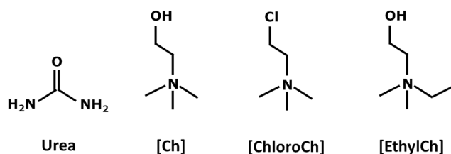
Scheme 1 Schematic structures of urea and the cations of the chloride-based salts investigated in this work. From left to right, urea, choline, chlorocholine, N -ethylcholine. Cations are labelled as [Ch], [ChloroCh], and [EthylCh], respectively.
