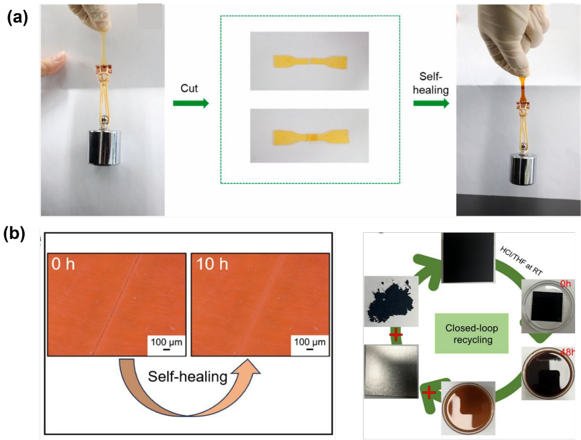
Fig.9 (a) Different self-healing test for silicone vitrimer matrix nanocomposite. Reproduced with permission from Ref. 164 Copyright 2022 Elsevier Ltd. (b) Self-healing and closed-loop recyclability of MWCNT reinforced epoxidized soybean oil-based vitrimer nanocomposite. Reproduced with permission from Ref. 226 Copyright 2024 American Chemical Society.
