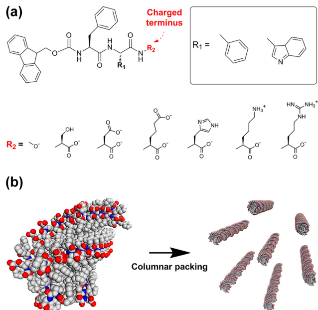
Fig. 28 (a) Amphoteric peptide molecular structure. (b) Illustration of the highly charged hexagonal liquid-crystalline phase with a large d spacing during the hierarchical chiral self-assembly of the peptides. Adapted with permission from ref. 296. Copyright 2018 American Chemical Society.
