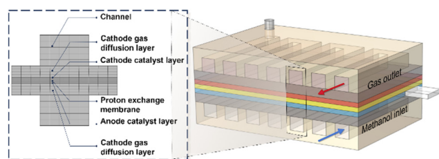
Fig. 1 3D geometric model of DMFC.
