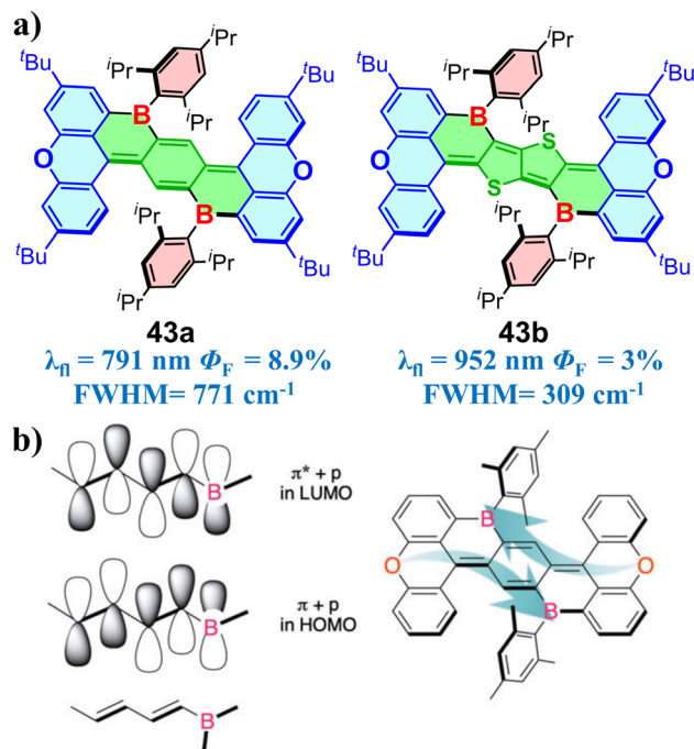
Fig. 12 (a) NIR emissive OBCTs with fused aromatic \pi -bridges based on an electron push-pull effect. (b) Illustration showing the orbital interaction of FMOs and the push-pull effect in 43a . Copyright 2021, John Wiley & Sons.
