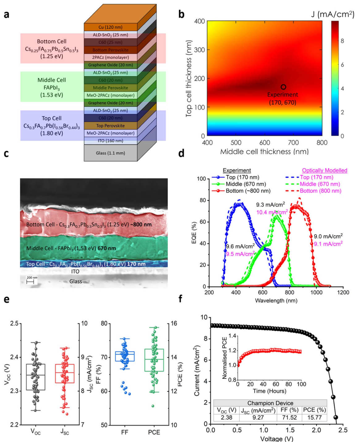
Fig. 2 Demonstration of monolithic PPP triple-junction solar cells together with optical modelling analysis. (a) Schematic diagram of the entire device stack, (b) optically modelled J_{\text{sc}} heatmap of the top and middle subcell perovskite absorber thickness variation based on the stack shown in (a). Note that the optical modelling range for the top and middle perovskite absorber layers are 0–400 nm and 400–800 nm, respectively, with a fixed bottom layer thickness of 800 nm, (c) corresponding high-resolution cross-sectional SEM image, (d) EQE showing each of the three subcells including the integrated EQE- J_{\text{sc}} and optically modelled EQE with the same subcell absorber thicknesses. In addition, the optically modelled EQE for the maximum point (180 nm, 580 nm) in the heatmap in (c) is shown in ESI Fig. 13b,† (e) photovoltaic characteristics ( V_{\text{oc}} , J_{\text{sc}} , FF, and PCE) for the batch, and f. Reverse J - V of the champion device (inset: 100 hours stability measurement). Note, the photovoltaic data consisted of seven substrates (8 cells each).
