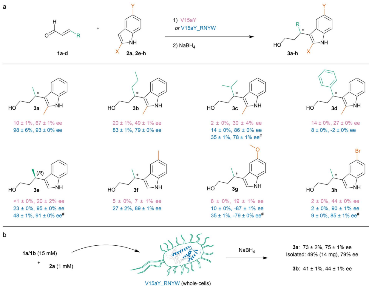
Scheme 2 (a) Substrate scope of the enantioselective vinyllogous FC-alkylation reaction catalysed by V15aY and V15aY_RNYW. Reaction conditions (unless otherwise noted): V15aY variant (60 \mu M dimer concentration), 1a–d (5 mM), 2a, 2e–h (1 mM) in MES buffer (20 mM, pH 5.5), containing NaCl (150 mM) and DMF (8% v/v) in a total volume of 300 \mu L, continuously inverted for 16 h at 8 ^{\circ} C. For 3a–d and 3f–h , ee is assigned relative to the enantiomer obtained with V15aY, in which the “–” symbol represents the opposite enantiomer. For 3e , absolute configuration is assigned by comparison of order of elution on HPLC with the literature and previous work. 16,42 # Performed using 25 mM 1 , see Table S5† for results of reactions performed at 25 ^{\circ} C. (b) Whole-cell catalysis and application on millimolar scale. Reaction conditions: washed whole-cells expressing V15aY_RNYW (6 OD 600 units), 1a/1b (15 mM), 2a (1 mM) in MES buffer (20 mM, pH 5.5), containing NaCl (150 mM) and DMSO (8% v/v) in a total volume of 300 \mu L, continuously inverted for 21 h at 8 ^{\circ} C. Results are based on at least three experiments, using two or more independently produced batches of protein, or three independent cultures of whole-cells. Errors are the standard deviation of the results. See ESI† sections 9 and 11 for more details.
