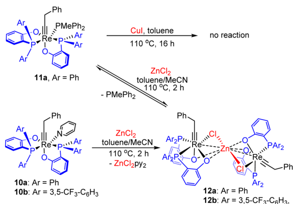
Scheme 2 Attempted extraction of \text{PMePh}_2 from \text{Re}(\equiv\text{CCH}_2\text{Ph})(\text{ArPO})_2 with 3d transition metal salts.
