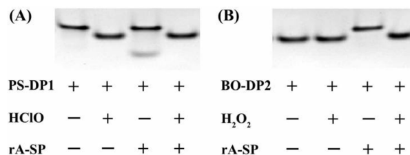
Fig. 3 PAGE characterization of (A) HClO 2 - and (B) H 2 O 2 -induced activation of the DNase activity.
