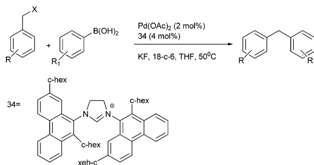
Scheme 43
