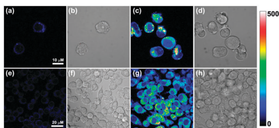
Fig. 104 Top: structure of CM1 and CM2 and the mechanism of their reaction with \text{ClO}^- . Bottom: (a) fluorescence images of HL-60 cells with CM1 (b) bright-field images of cells in panel (a). (c) After addition of \text{H}_2\text{O}_2 (d) bright-field images of cells in panel (c). (e) Fluorescence images of RAW264.7 cells with CM1 (f) bright-field images of cells in panel (e). (g) Cells loaded with CM1 then LPS (h) bright-field images of cells in panel (g). Image reproduced with permission. 329
