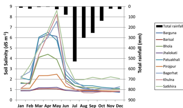
Fig. 2 Seasonality of soil salinity (district average) and total rainfall (study area). Data shown for 2009 as an illustration (see Section 3a for more details).
