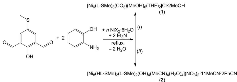
Scheme 1 Synthesis of the hexanuclear and octanuclear nickel(II) Schiff-base complex compounds 1 and 2 . Reaction conditions: (i) n = 2 for \text{X} = \text{Cl} and \text{MeOH} : \text{THF} = 4 : 1 ; (ii) n = 1.4 for \text{X} = \text{NO}_3 and \text{MeCN} : \text{PhCN} = 10 : 1 . For the IR spectra of these compounds, see Fig. S3 and S4.†
