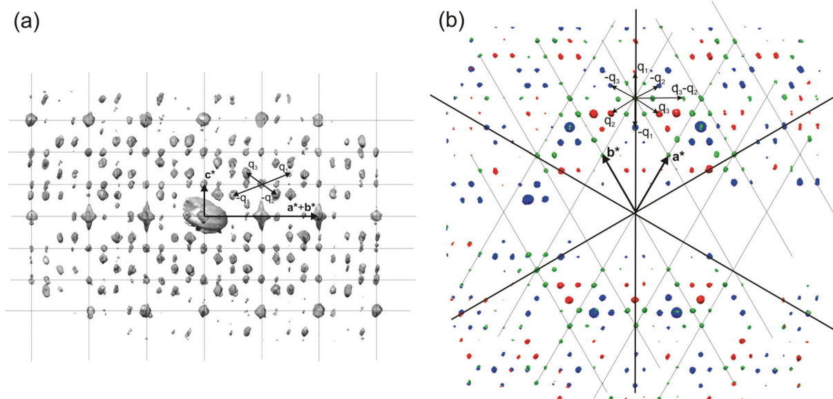
Fig. 9 3D distribution of diffracted intensities in the reciprocal space. (a) Projection along a^*-b^* with the basic unit cell and modulation vectors is indicated. Vectors \mathbf{q}_3 and -\mathbf{q}_2 point partly toward the reader (cf. part b of this figure); other vectors lie in the plane of the drawing. (b) Three layers viewed along c^* . Blue, l = 2/3 ; green, l = 1 ; red, l = 4/3 . Reproduced with permission from ref. 101. Copyright 2011 American Chemical Society.
