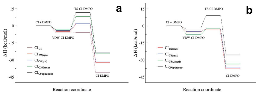
Fig. 4 Reaction energy profiles of the CI + DMPO → CI-DMPO reactions of \text{Cl}_{\text{C1}} , \text{Cl}_{\text{C2}} , \text{Cl}_{\text{C4}} , \text{C}_{9\beta\text{pin}} and \text{Cl}_{\text{C3Al}} , calculated starting from the more stable (a) and the less stable (b) conformation of each adduct.
