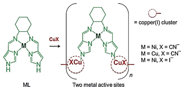
Scheme 3 Synthesis of [\text{NiL}]_2[\text{Cu(I)CN}]_9_n , [\text{Cu(II)L}]_2[\text{Cu(I)CN}]_9_n and [\text{NiL}][\text{Cu(I)I}]_2_n . [Reproduced from ref. 101 with permission from The Royal Society of Chemistry.]
