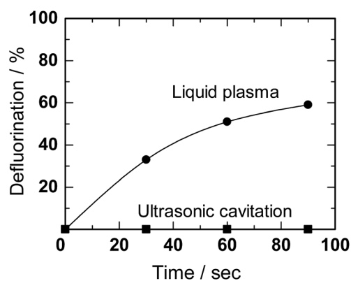
Fig. 20 Defluorination yields (%) from the degradation of aqueous PFOA solutions (0.01 mM) by ultrasonic cavitation alone and by the microwave discharge in-liquid plasma method under simultaneous ultrasonic cavitation (MW power, 220 W; power for cavitation, 90 W). Reproduced from Horikoshi et al. 156 Copyright 2017 by Elsevier.
