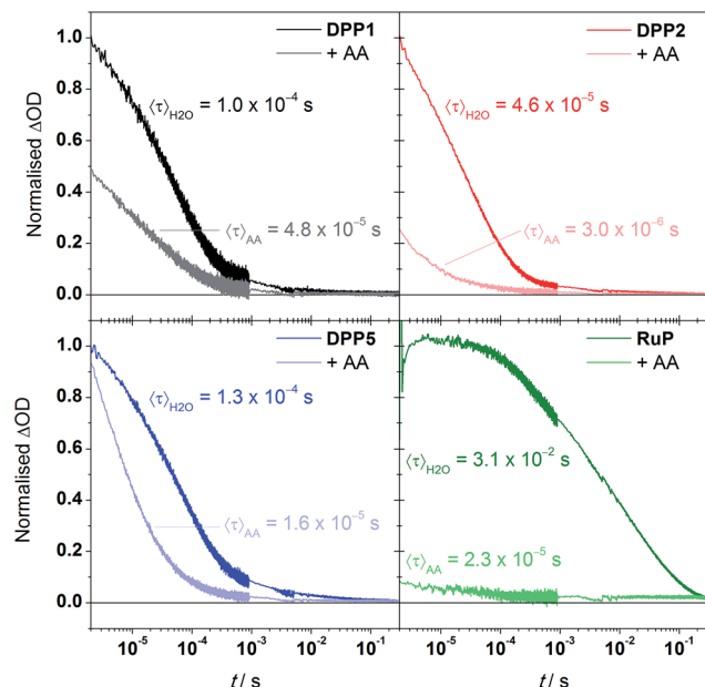
Fig. 5 Normalised change in absorbance at 700 nm in H 2 O or AA solutions (10 mM, pH = 4.5) of dye-sensitised TiO 2 thin films. Traces were normalised to the amplitude observed in H 2 O at 2 μs for the DPP dyes, and 3 μs for RuP. Characteristic mean lifetimes are indicated near the corresponding trace.
