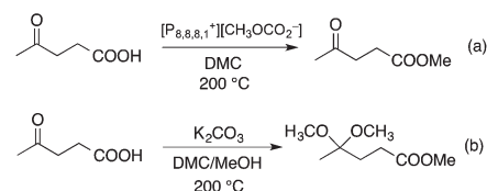
Scheme 8 Alkylation reactions of levulinic acid with dimethyl carbonate.
