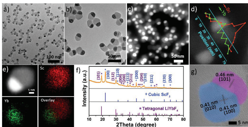
Fig. 1 (a, b) TEM images and (c) HAADF-STEM image of \text{ScF}_3 - \text{LiYbF}_4 Janus NPs, (d) EDS line scan and (e) STEM-EDS elemental mapping of a single NP, which indicates the Sc and Yb elements are located in the cubic and hemispherical region, respectively. (f) XRD patterns of as-synthesized \text{ScF}_3 - \text{LiYbF}_4 Janus NPs, and (g) HRTEM image of \text{ScF}_3 - \text{LiYbF}_4 Janus NPs. Standard cubic \text{ScF}_3 (ICDD: 00-046-1243) and tetragonal \text{LiYbF}_4 (ICDD: 01-071-1211) patterns are also shown in (f).
