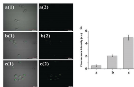
Fig. 106 Confocal fluorescence images of RAW 264.7 cells: (a) RAW 264.7 cells stained with 64 (5 \mu\text{M} ) for 15 min. (b) RAW 264.7 cells stimulated with 1 \mu\text{g mL}^{-1} LPS and 50 ng \text{mL}^{-1} IFN- \gamma for 4 h, and then 10 nM PMA for 30 min before incubation with 64 (5 \mu\text{M} ) for 15 min. (c) RAW 264.7 cells stained with 64 (5 \mu\text{M} ) for 15 min and then ONOO ^{-} (10 \mu\text{M} ) was added for 20 min. (d) Relative fluorescence intensity of cells in panels (a–c). (1) Overlay field. (2) Green channel. Green channel: 460–540 nm, excitation at 404 nm. Copyright 2018 Royal Society of Chemistry.
