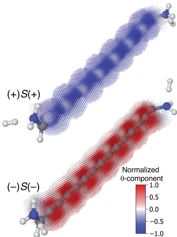
Fig. 10 Current density calculated at the Fermi energy for the (+)\text{S}(+) and (-)\text{S}(-) conformations of 1,15-diamino-[14]cumulene; the 15-carbon cumulene with helical \pi -orbitals. The vector field is calculated on a high-density grid and coloured by the \theta -component.
