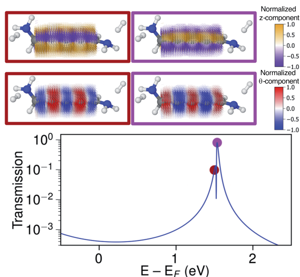
Fig. 9 Transmission calculated with s-band electrodes and current density calculated around the LUMO resonance energy for the (-)\text{S}(-) conformation of 1,5-diamino-[4]cumulene. The current density vector field is shown on a high-density grid and is coloured by the z -component (first row) and by the \theta -component (second row). In the transmission plot coloured dots indicate the energy at which the current density is calculated.
