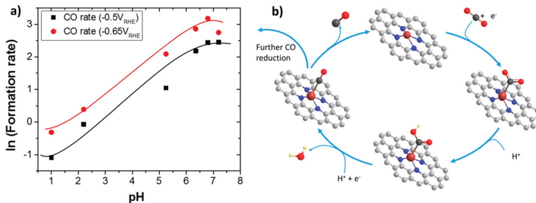
Fig. 25 (a) pH dependence of the CO formation rate at a constant potential on the RHE scale (black, -0.5 \text{ V}_{\text{RHE}} ; red, -0.65 \text{ V}_{\text{RHE}} ); (b) scheme of the proposed catalytic cycle of the \text{CO}_2\text{RR} on Fe-N-C catalysts. Adapted with permission from ref. 349. Copyright 2018 American Chemical Society.
