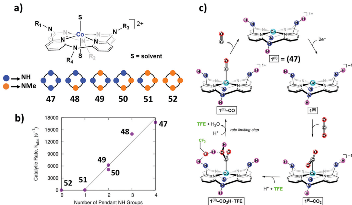
Fig. 16 (a) Sketch of the Co complexes 47–52 . (b) Experimental catalytic rate constants, k_{obs} ( s^{-1} ), as a function of the number of pendant secondary amines for complexes 47–52 measured in the presence of 1.5 M TFE and under CO 2 saturation at a scan rate of 0.1 V s^{-1} . Rates are obtained from the plateau current. A linear fit ( R^2 = 0.97 ) is shown in gray for complexes 47–52 . (c) Proposed EEC catalytic cycle illustrated with complex 1 (0) = 47 where E = electrochemical, and C = chemical step. Adapted with permission from ref. 257. Copyright 2018 American Chemical Society.
