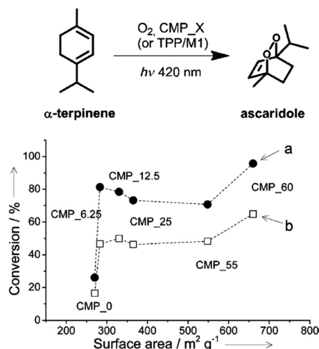
Fig. 17 Porosity control of CPPs by the silica template. Photocatalytic conversion of α-terpinene into ascaridole with poly(benzothiadiazole)s having difference surface areas. Photo-reactor set-up with (a) lower O 2 flow rate (5 mL min -1 ) and (b) higher O 2 flow rate (10 mL min -1 ). Adapted with permission. 22 Copyright 2013 Wiley-VCH.
