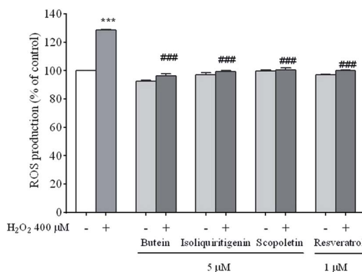
Fig. 4 The protective effects of 5 \mu\text{M} of butein, isoliquiritigenin, scopoletin, or 1 \mu\text{M} resveratrol on \text{H}_2\text{O}_2 -induced ROS production. The data are shown as mean \pm S.E.M. of three independent experiments ( ***p < 0.001 vs. control; ###p < 0.001 vs. 400 \mu\text{M} \text{H}_2\text{O}_2 -treated group).
