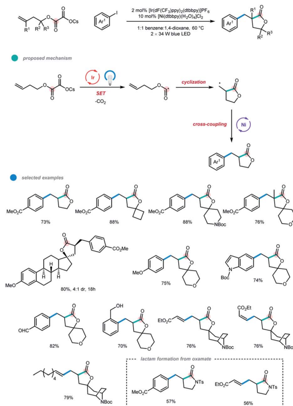
Scheme 4 Preparation of spiro-lactones by an alkoxy-carbonyl radical cyclization-cross-coupling cascade.
