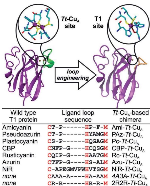
Fig. 1 X-ray crystallographic structures of native Tt -Cu A (PDB ID 2CUA) 38 on the left, and that of Ami- Tt -Cu A on the right (PDB ID 5U7N). 36 The loop replaced in the chimeras is indicated in green and orange, respectively. The loop sequences employed to obtain the different chimeras are listed below. Red letters denote the conserved ligand set.
