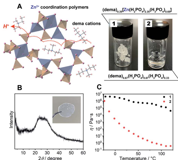
Fig. 1 (A) Schematic structure of 1 , the blue and orange polyhedra represent Zn 2+ and H 2 PO 4 − , the captured organic ions indicate dema cations. The formula and digital photographs of 1 and 2 at 25 °C. (B) The powder X-ray diffraction (PXRD) pattern of 1 . The inset shows a digital photograph of a monolith of 1 after annealing at 120 °C. (C) Temperature dependence of the viscosity of 1 (black) and 2 (red).
