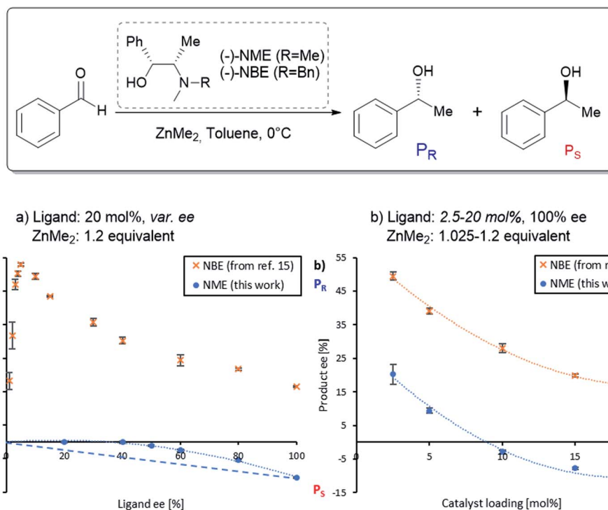
Fig. 2 (a) NLE-curve and (b) \text{ee}_P vs. catalyst loading-plot of the (–)-NME- (blue dots) and (–)-NBE- (orange crosses, from ref. 11) catalyzed enantioselective addition of \text{ZnMe}_2 to benzaldehyde at 0 °C. Each point is the mean of three independent experiments; the vertical bars depict standard deviations. The second-order polynomial fits (dotted lines) serve as visual guidelines. The dashed line in (a) simulates a linear \text{ee}_P/\text{ee}_L relationship for the NME-catalysed reaction. The product ee is defined as (P_R - P_S)/(P_R + P_S) .
