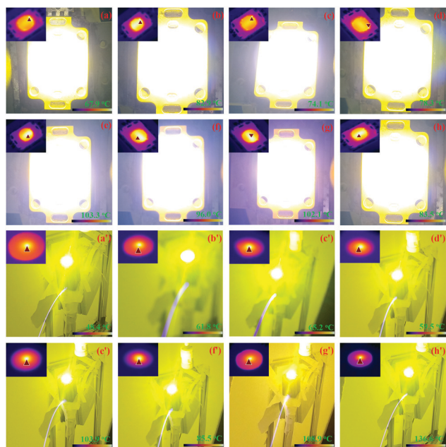
Fig. 5 Photographs of the lighting of white LEDs/LDs devices and corresponding infrared thermal images of (a/a') \text{PrO}_2\text{MnO}_8 , (b/b') \text{PrO}_2\text{MnO}_8 , (c/c') \text{PrO}_2\text{MnO}_8 , (d/d') \text{PrO}_2\text{MnO}_8 , (e/e') \text{PrO}_1\text{MnO}_6 , (f/f') \text{PrO}_1\text{MnO}_6 , (g/g') \text{PrO}_2\text{MnO}_8 , and (h/h') \text{PrO}_4\text{Mn}_{10} excited by blue LEDs/LDs.
