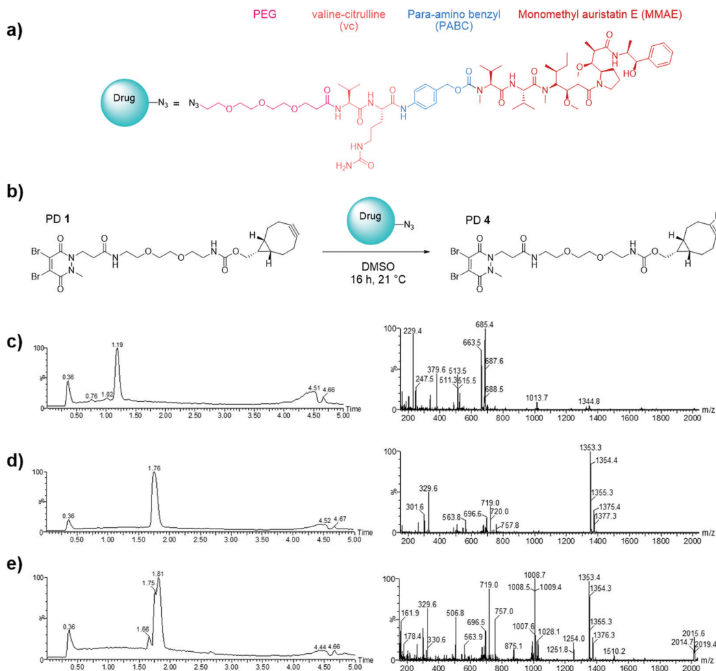
Fig. 6 Selection of drug for the generation of the hLRG1-targeting ADC. (a) Structure of \text{N}_3-\text{PEG}_3-\text{vc}-\text{PABC}-\text{MMAE} ; (b) SPAAC 'click' functionalisation (the pre-click strategy) reaction between the strained alkyne bearing PD 1 and azide-linked MMAE to form PD 4. (c) LCMS analysis of PD 1 (662 Da); (d) \text{N}_3-\text{PEG}_3-\text{vc}-\text{PABC}-\text{MMAE} (1353 Da) and (e) pre-click reaction of PD 1 with \text{N}_3-\text{PEG}_3-\text{vc}-\text{PABC}-\text{MMAE} showing formation of PD 4 (2015 Da) and complete consumption of PD 1.
