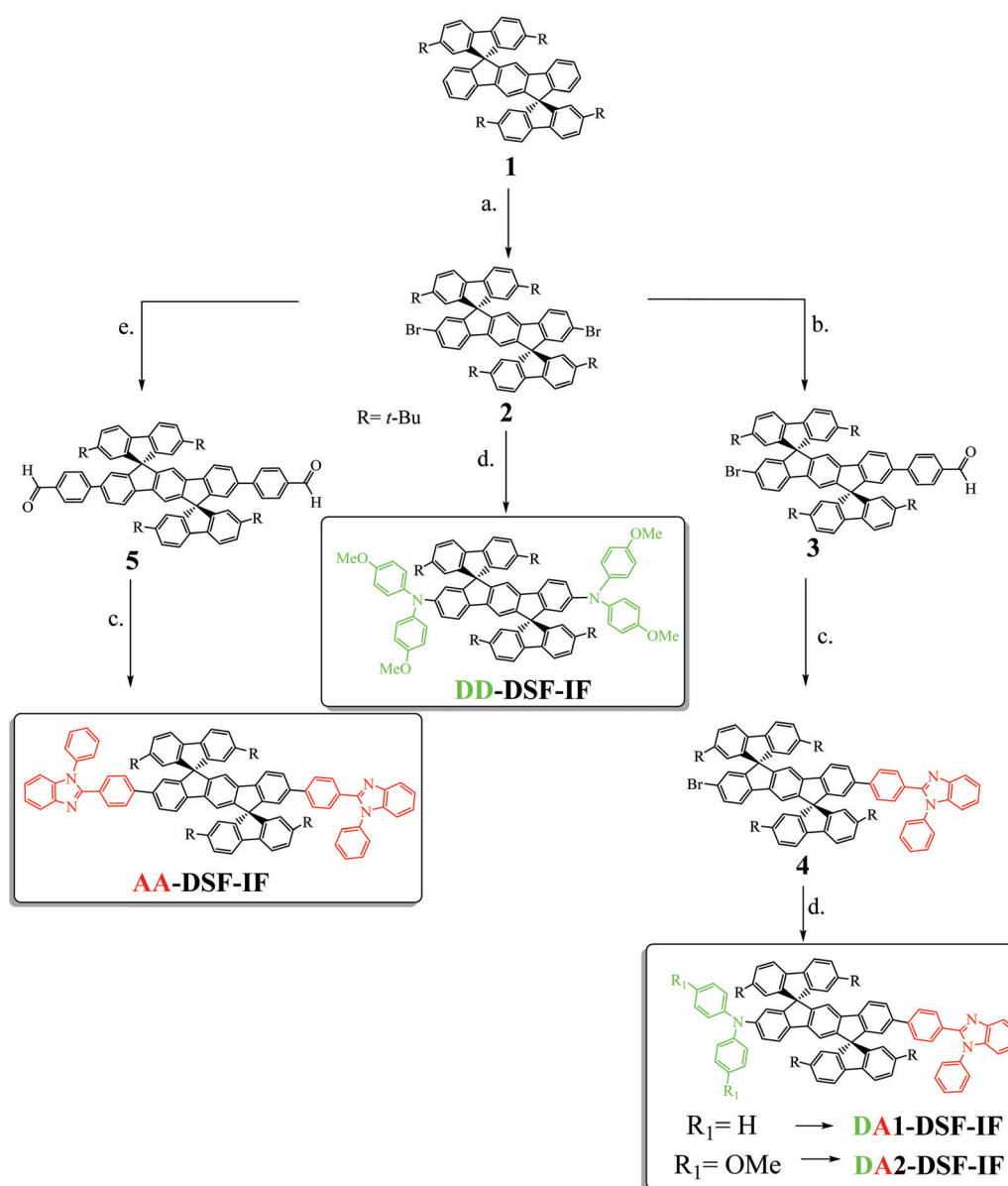
Scheme 1 Synthesis of DA1-DSF-IF , DA2-DSF-IF , AA-DSF-IF and DD-DSF-IF . (a) Br 2 , Na 2 CO 3 , I 2 (catalytic amount), CH 2 Cl 2 /Water, rt, (90%); (b) Pd 2 (dba) 3 /P( t -Bu) 3 , Na 2 CO 3 , 4-formylbenzeneboronic acid (1.4 eq. vs. 2 ), toluene/water (6/1), 100 °C, (30%); (c) methoxyethanol, N -phenyl- o -phenylenediamine, 120 °C (70% for AA-DSF-IF and 65% for 4 ); (d) Pd(OAc) 2 , P( t -Bu) 3 , t -BuOK, diphenylamine for DA1-DSF-IF or 4,4'-dimethoxydiphenylamine for DA2-DSF-IF , toluene, 100 °C (<10% for DA1-DSF-IF , 50% for DA2-DSF-IF and 50% for DD-DSF-IF ); (e) Pd 2 (dba) 3 , P( t -Bu) 3 , Na 2 CO 3 , 4-formylbenzeneboronic acid (2 eq. vs. 2 ), toluene/water, 100 °C, (85%).
