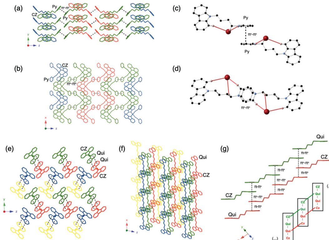
Fig. 1 Different crystal views of the intermolecular packing of Py-Br (a and b) and Qui-Br (e and f). (c and d) Molecular \pi-\pi^+ and \pi^+-\pi^+ interactions in Py-Br . (g) Molecular \pi-\pi^+ and \pi^+-\pi^+ interactions in Qui-Br .
