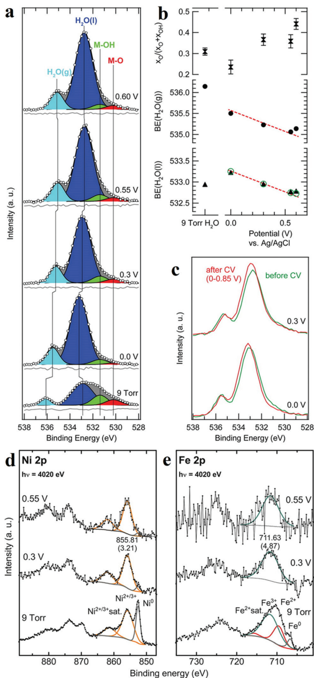
Fig. 6 (a) Normalized and background-subtracted O 1s XPS spectra of Ni-Fe electrocatalyst. (b) Fit results for spectra in (a): relative intensity of the M-O component in the MO x (OH) y catalyst and measured H 2 O peak positions (black symbols). (c) Comparison of XPS measurements taken at identical applied potentials before (green) and after (red) the second electrochemical conditioning. Normalized XPS spectra of (d) Ni 2p and (e) Fe 2p transitions for a Ni-Fe electrocatalyst. 61
