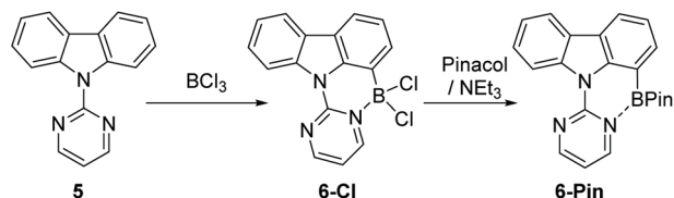
Scheme 3 Pyrimidine directed carbazole borylation.
