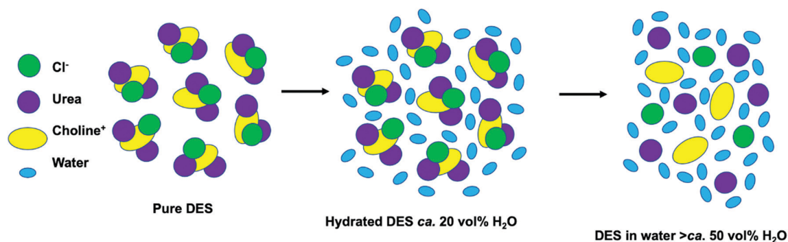
Fig. 16 Cartoon diagram showing structural changes in a DES starting with the pure choline \text{Cl} :urea DES (left). As the water content increases the hydrated DES regime is reached (middle, ca. 20 vol%), then the high concentration regime where everything is fully hydrated (ca. 50 vol%). Reprinted with permission from Elsevier. 207
