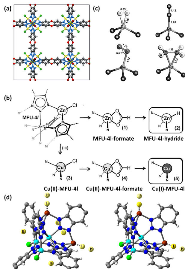
Fig. 7 (a) The structure of MFU-4l, (b) schematic representation of the conversion of MFU-4l into its corresponding hydride-containing and \text{Cu(I)} -containing compounds, and (c) binding geometries for \text{H}_2 , \text{N}_2 , \text{O}_2 and \text{C}_2\text{H}_4 at the \text{Cu(I)} site as determined by DFT calculations. (d) \text{D}_2 binding sites for \text{Cu(I)-MFU-4l} determined at 7 \text{ K} by NPD experiments at a 0.75 \text{ D}_2/\text{Cu} at the dosing temperatures of 40 \text{ K} (left) and 77 \text{ K} (right). Reprinted with permission from ref. 55a and b. Copyright 2014, Wiley. Copyright 2021, American Chemical Society.
