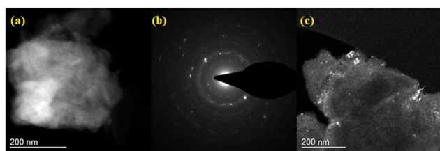
Fig. 3 (a) HADF-STEM image of C50 carbon. (b) SAED pattern acquired over an area of 200 nm. (c) HADF-STEM image of the C-50 sample selecting the reflection at d = 0.31 \text{ nm} in the SAED pattern.
