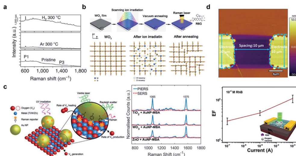
Fig. 1 Vacancy-induced SERS-active semiconductor substrates. (a) SERS spectra of R6G on pristine and Ar/H_2 -treated W_{18}O_{49} . Reproduced with permission from ref. 26. Copyright 2015, Springer Nature. (b) Fabrication and SERS evaluation of ion-irradiated WO_3 thin films. Reproduced with permission from ref. 31. Copyright 2017, American Chemical Society. (c) Schematic illustration of the PIERS technique and SERS performance of semiconductors before and after UV irradiation. Reproduced with permission from ref. 32. Copyright 2019, John Wiley and Sons. (d) AFM topographical image and SERS evaluation of the electrically tuned WO_3 substrate. Reproduced with permission from ref. 36. Copyright 2019, American Chemical Society.
