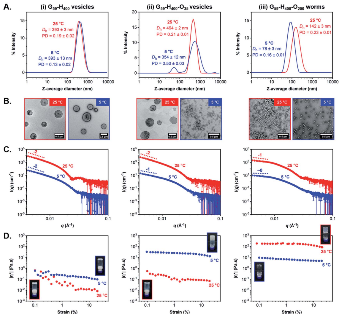
Fig. 5 Characterization data obtained for (i) G_{59} - H_{400} diblock copolymer vesicles, (ii) G_{59} - H_{400} - O_{35} triblock copolymer nano-objects, and (iii) G_{59} - H_{400} - O_{200} triblock copolymer nano-objects at 25 °C (red data) and 5 °C (blue data) after incubation at each temperature for 24 h prior to analysis: (A) intensity-weighted particle size distributions, mean D_h values and polydispersities determined by DLS analysis of 0.1% w/w aqueous dispersions (the error indicates the standard deviation from at least three repeat measurements). (B) Representative TEM images obtained using a uranyl formate stain. (C) SAXS patterns recorded for 1.0% w/w aqueous dispersions. (D) Complex viscosity ( |\eta^*| ) as a function of applied strain (insets show digital images recorded for the corresponding aqueous copolymer dispersions at 10–11% w/w solids, which indicate whether they form a free-standing gel or a free-flowing fluid in each case).
