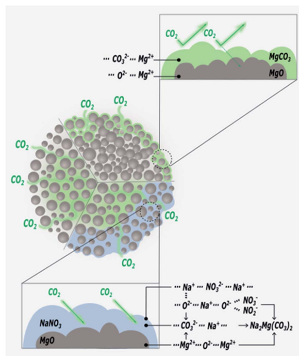
Fig. 7 The role of the MgO sorbent with nitrate salts for improving CO 2 capture capacity.
