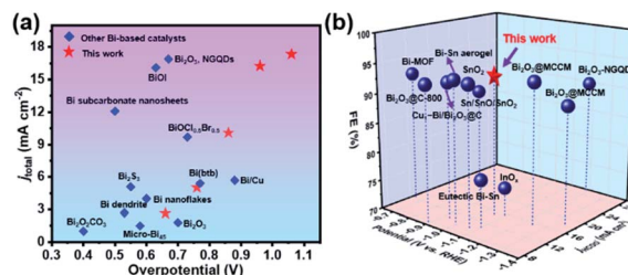
Fig. 3 (a) Literature overview of Bi-based electrocatalysts for the \text{CO}_2 -to-formate conversion. Overpotentials ( \eta ) calculated using the equilibrium potential for \text{CO}_2/\text{HCOO}^- , E = -0.2 V vs. RHE. 34 (b) Comparison of partial current density and FE of formate for the SU-101 NRs with those of previously reported Bi-based and other advanced catalysts at the applied potentials.
