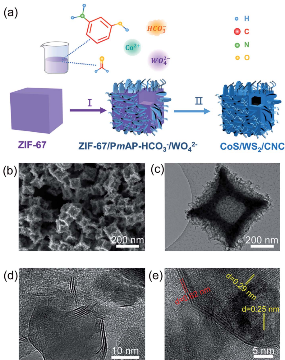
Fig. 1 (a) Schematic illustration of the fabrication pathway of CoS/WS 2 /CNC. (b) SEM, (c) TEM, (d) TEM, and (e) high-resolution TEM images of CoS/WS 2 /CNC-1.
