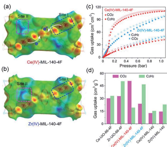
Fig. 19 The electrostatic potential distributions on the Hirshfeld surface of (a) \text{Ce-MIL-140-4F} and (b) \text{Zr-MIL-140-4F} (red-to-blue color indicates the high-to-low transition of electron density); (c) the \text{CO}_2 and \text{C}_2\text{H}_2 isotherms of \text{Ce(IV)-} and \text{Zr(IV)-MIL-140-4F} collected at 298 K; (d) the \text{CO}_2 and \text{C}_2\text{H}_2 uptakes of different MOF samples at 298 K. Reprinted with permission from ref. 30. Copyright 2021, WILEY-VCH Verlag GmbH.
