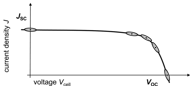
Fig. 5 Schematic of a JV curve with possible operating points for IS measurements, V_{\text{OC}} , J_{\text{SC}} and MPP plus around the MPP. The points within the ellipses signify the essential steady-state operating point and the ellipses themselves indicate the range of voltage and current density that the devices undergo during the IS measurement, respectively.
