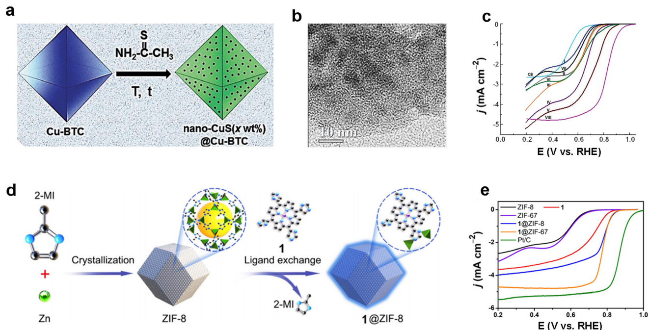
Fig. 11 MOF-based ORR electrocatalysts. (a) Schematic diagram of the synthesis of CuS(x wt%)@Cu-BTC nanoparticles; (b) TEM images of nano-CuS(28 wt%)@Cu-BTC; (c) LSV curves of nano-CuS(28 wt%)@Cu-BTC and other samples for ORR tests in O 2 -saturated 0.1 M KOH, rotation rate: 1600 rpm. Reproduced with permission. 97 Copyright 2016, Wiley-VCH; (d) schematic diagram of the preparation of 1@ZIF-8; (e) LSV curves of 1@ZIF-8 and other samples for ORR tests in O 2 -saturated 0.1 M KOH, rotation rate: 1600 rpm. Reproduced with permission. 98 Copyright 2021, Wiley-VCH.
